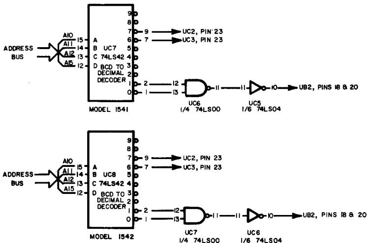
Fig. 7-44. RAM/VIA address decoder changes, Model 1542.
